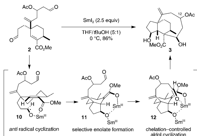
Scheme 3. A \text{SmI}_2 -mediated dialdehyde cyclization cascade for the stereocontrolled construction of the pleuromutilin framework.
