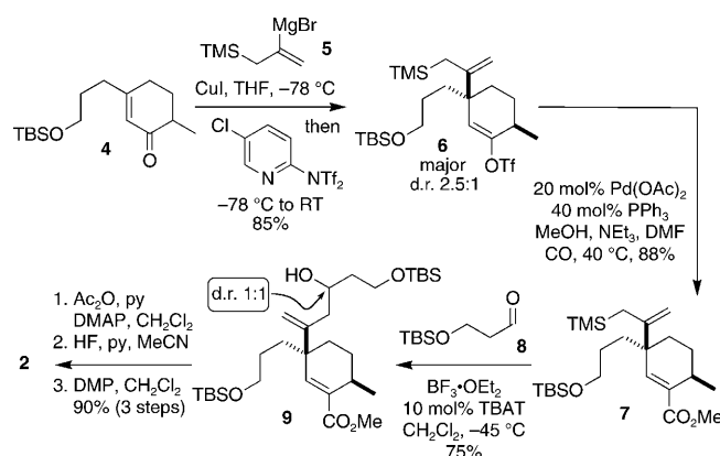
Scheme 2. Synthesis of dialdehyde cyclization substrate 2 .
